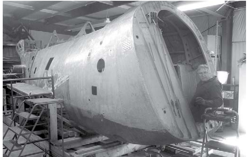
Team leader Paul Blinn leads the paint stripping process and inspection of the rear fuselage of the H44 helicopter restoration.
